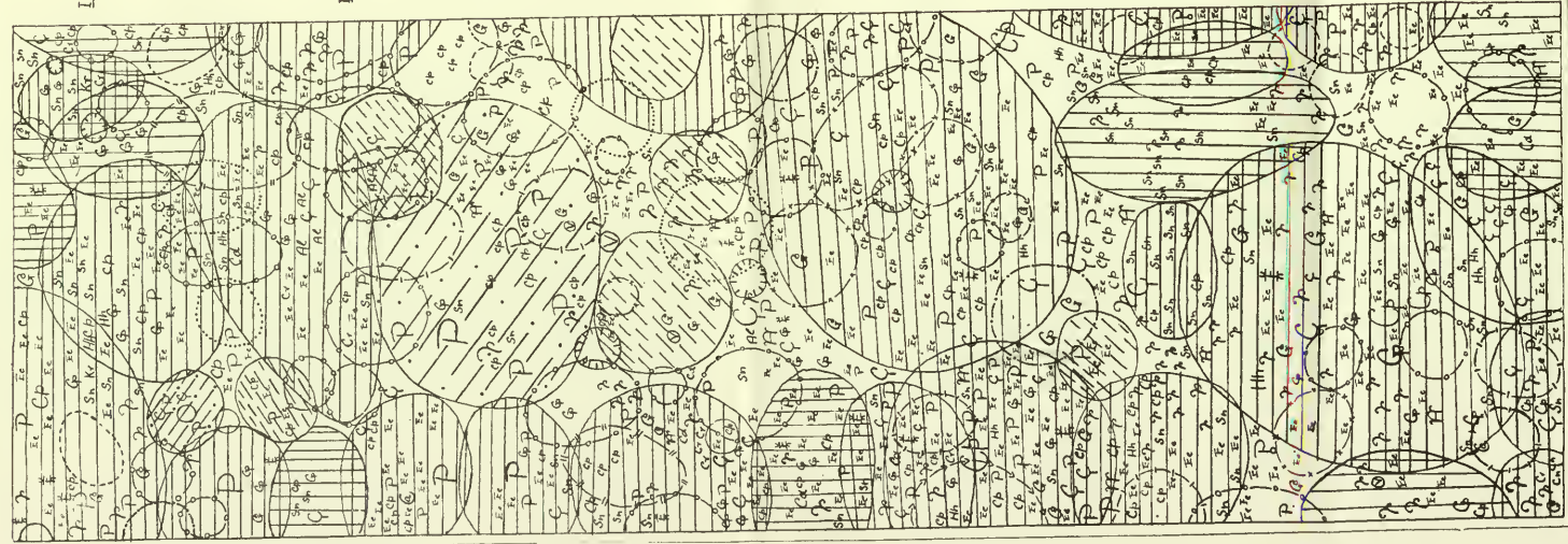
Belt Transect showing three discontinuous layers of vegetation and the size and spacing of the individual plants.
